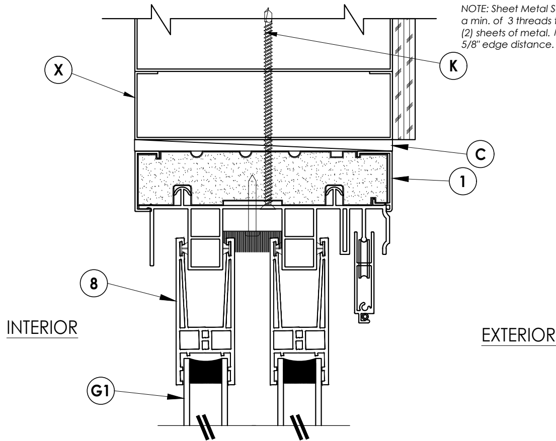
2 VERTICAL CROSS SECTION 3 Shown w/ Steel Stud framing option
